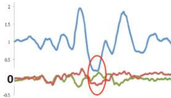
Figure 9 : Detection of Pothole using algorithm G-ZERO. Events are represented by tuple of measurements with all three axis values below specific threshold level.
