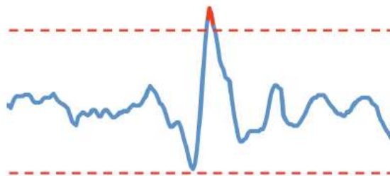
Figure 6: Pothole detection algorithm Z-THRESH. Events are represented by measurements with values exceeding specified threshold levels.
