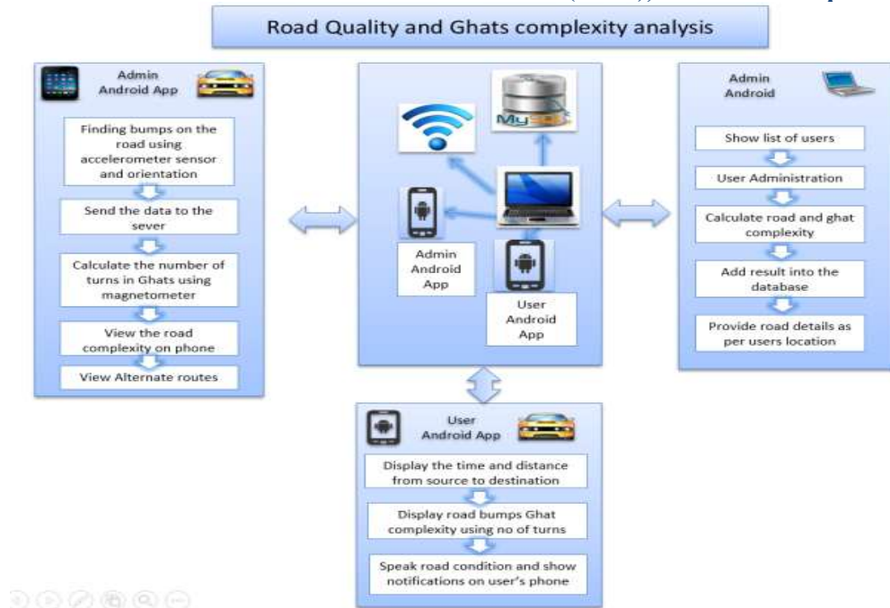
Figure 1: System Architecture Design
